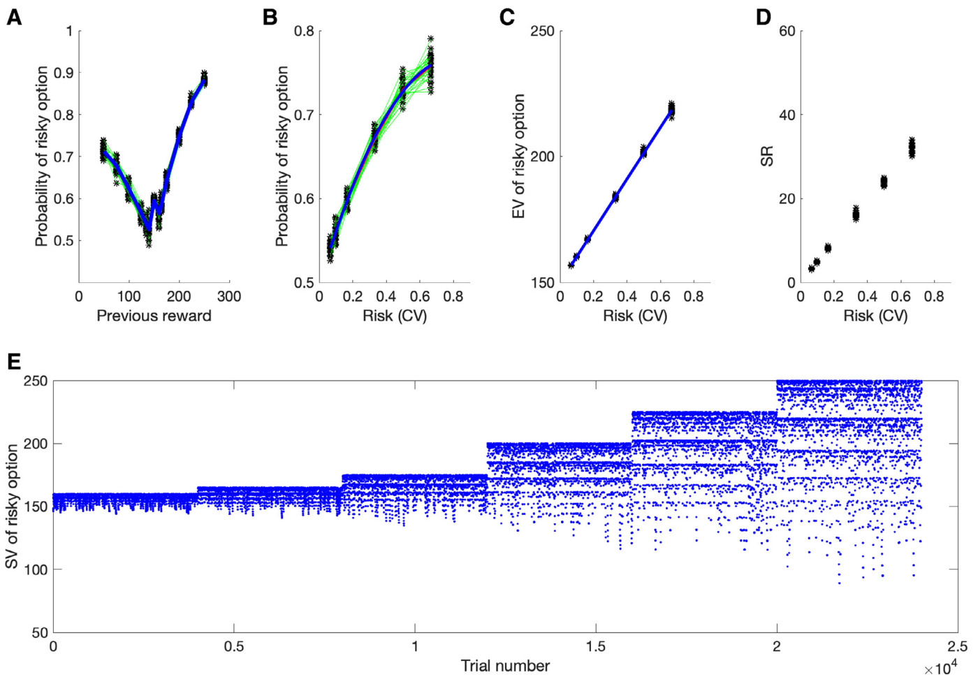
Fig. 3. The risk-seeking behavior captured by two-stage model. (A) The probability of risky choice over previous reward shows an asymmetric check marker. (B) The probability of risk choice as an increasing function of risk. (C) The mean of subjective value of the risky option is an increasing function of risk. (D) The subjective risk is an increasing function of risk. (E) The subjective value of risky option varies with the simulation trials in one session. The parameters are chosen as: \alpha_+ = 0.8 , \alpha_- = 0.15 , \theta = 300 , \lambda = 15 . The green lines denote one session while blue line denotes average over sessions.
