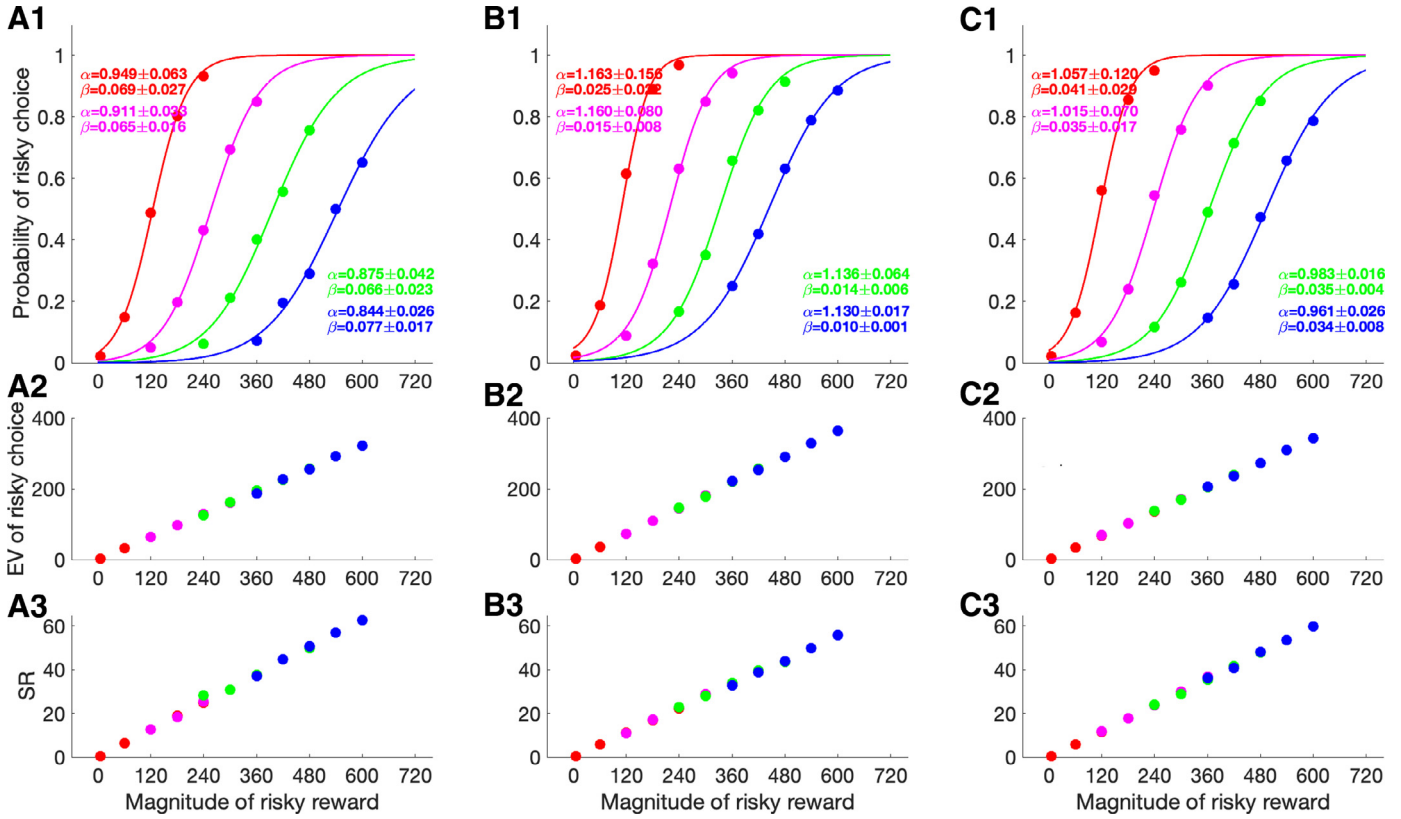
Fig. 5. Simulated risk behavior on tasks with fixed CV but variant average reward. The sensitivity and wealth/thirst parameters are set as: \lambda = 20 , \theta = 240 . The learning rates are set as \alpha_+ = 0.09 , \alpha_- = 0.078 in (A), \alpha_+ = 0.09 , \alpha_- = 0.058 in (B), and \alpha_+ = 0.09 , \alpha_- = 0.068 in (C). The dots in figures are simulated data and the lines are fitted choice probability based one expected utility function. The color denotes the magnitude of certain reward, red for 60, magenta for 120, green for 180, and blue for 240. The top panels show the fitted choice function for each condition with different learning rates. Middle panels show the average of subjective value of each risky option. Bottom panels show the subjective risk of each risky option. (A) Risk-avoiding behavior. The utility function parameters \alpha < 1 for all conditions. (B) Risk-seeking behavior. The utility function parameters \alpha > 1 for all conditions. (C) Risk-switching behavior: seeking small risk but avoiding large risk. The utility function parameter changes from \alpha > 1 to \alpha < 1 along with the increase of the risk.
