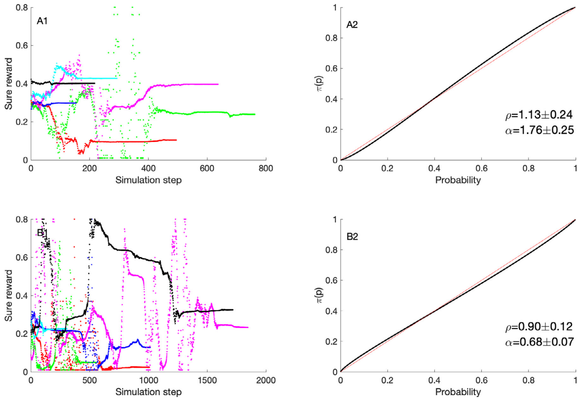
Fig. 9. Weighting of probability in simulated PEST task. (A1). The time course of the sure reward in an example trial of certainty equivalent searching task given \alpha_+ = 0.05 , \alpha_- = 0.02 , \lambda = 4 , and \beta = 0 . (A2) The weighting function of probability underweighting small probability and overweighting large probability. (B1) The time course of the sure reward in an example trial of certainty equivalent searching task given \alpha_+ = 0.02 , \alpha_- = 0.04 , \lambda = 4 , and \beta = 0 . (B2) The weighting function overweighting small probability and underweighting large probability.
