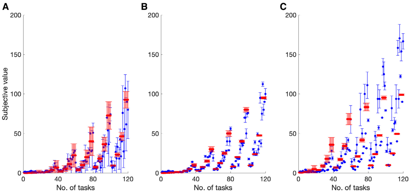
Fig. 7. Subjective value of each gamble. (A) \alpha_+ = 0.2, \alpha_- = 0.3 ; (B) \alpha_+ = 0.01, \alpha_- = 0.01 ; (C) \alpha_+ = 0.1, \alpha_- = 0.02 . Red for gamble (p_1, x_1) and blue for gamble (p_2, x_2) , dots denote the average of subjective value and bars denote the subjective risk.
