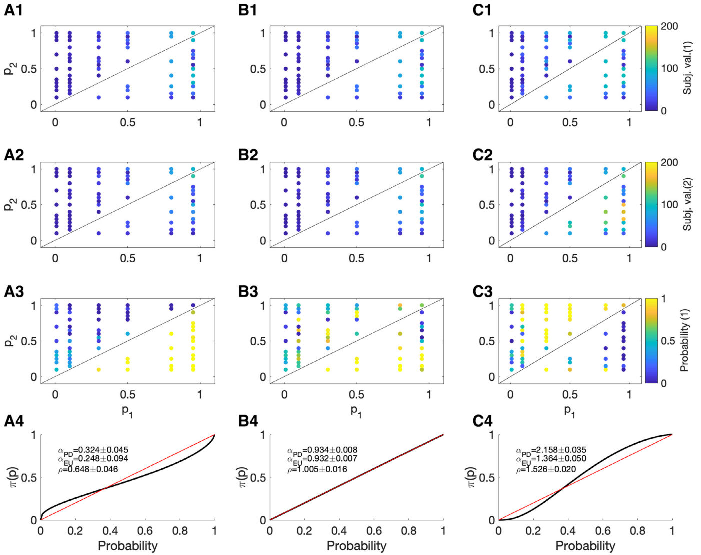
Fig. 8. Weighting of probability inferred from simulated choices. (A) Overweighting small probability but underweighting large probability. (B) Linear weighting of probability. (C) Underweighting small probability but overweight large probability. Black line is weighting function and red line is diagonal line. \rho is parameter of Prelec function \pi(p) = 1/\exp[-(-\ln p)^\rho] , \alpha_{PD} is parameter of utility function used by Hsu et al. [8], \alpha_{EU} is parameter of utility function in expected utility theory. The first and second row show the subjective value of gamble 1 and gamble 2, respectively. The third row shows the probability to choose gamble 1. The fourth row shows the weighting of probability.
